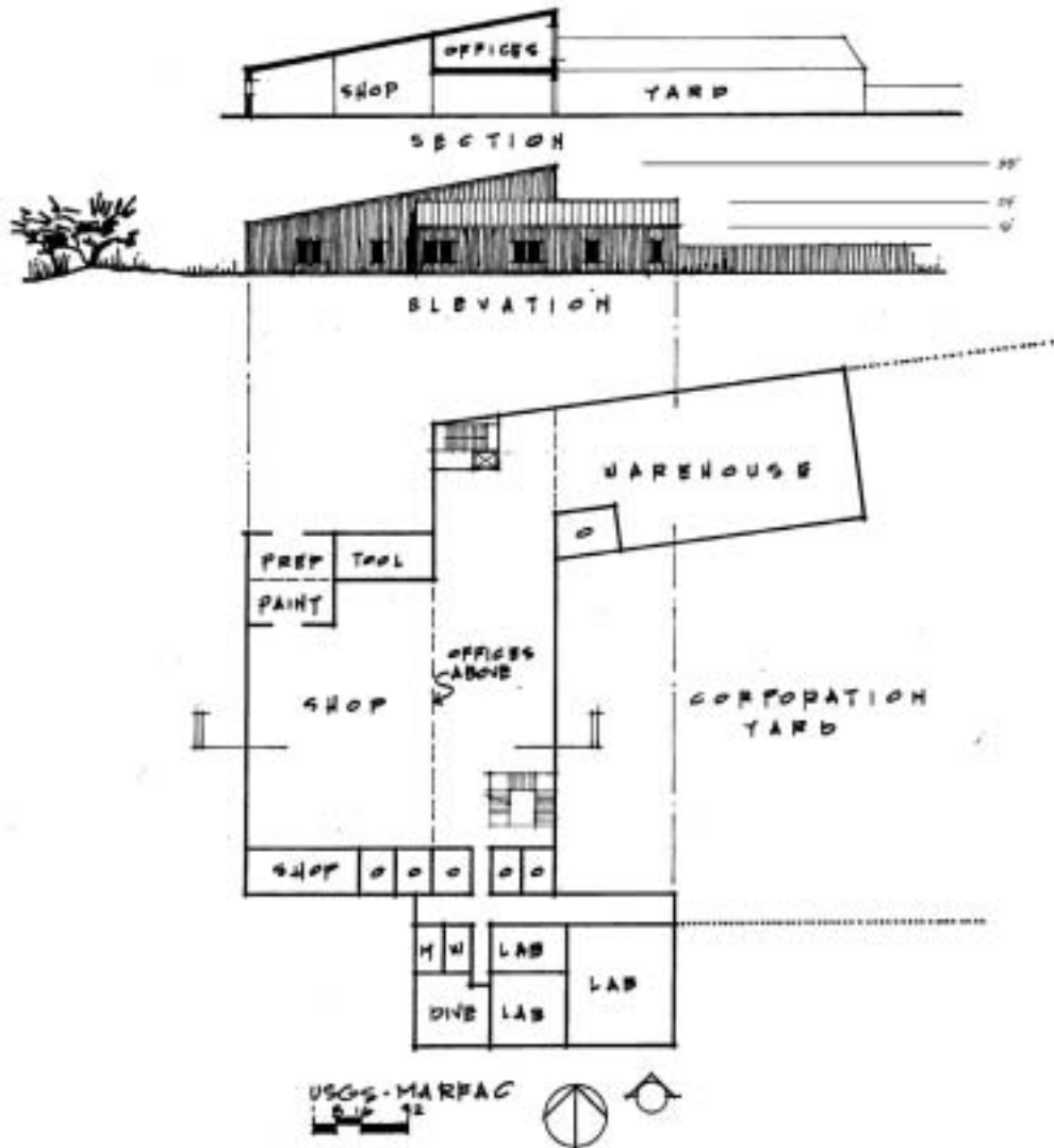
Fig. 7.9 Shared Warehouse, Shop, and Laydown Facility
