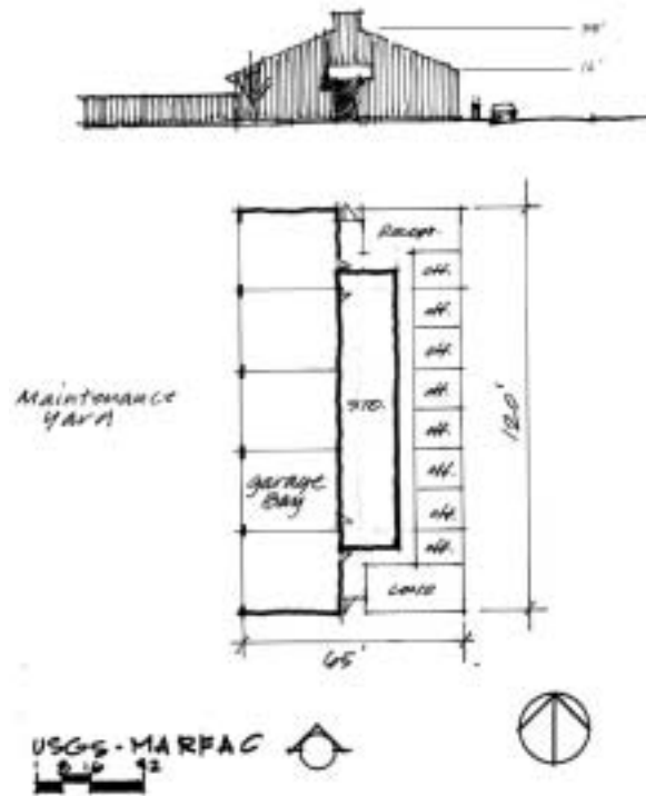
Fig. 7.10 Shared Warehouse, Shop, and Laydown Facility
