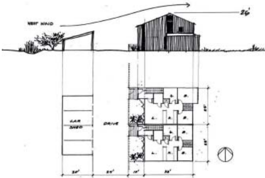
Fig. 7.12 Apartment/Townhouse Layout
